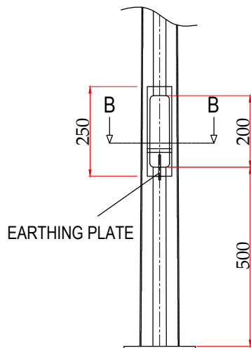
FUSE DETAIL
