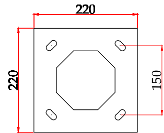
BASE PLATE
